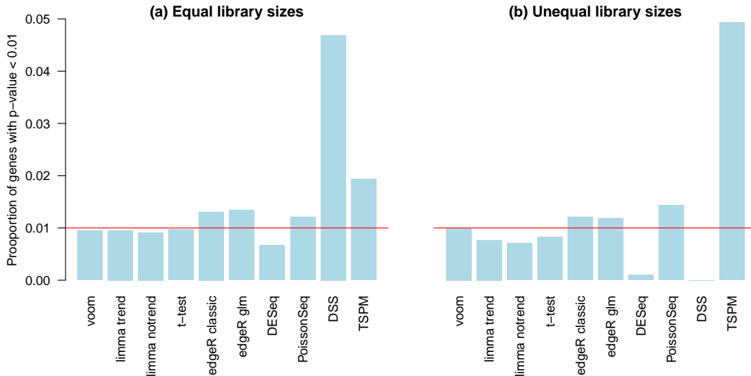
Figure 3: Type I error rates in the absence of true differential expression. The barplots show the proportion of genes with p-value < 0.01 for each method (a) when the library sizes are equal and (b) when the library sizes are unequal. The red line shows the nominal type I error rate of 0.01. Results are averaged over 100 simulations. Methods that control the type I error at or below the nominal level should lie below the red line.
