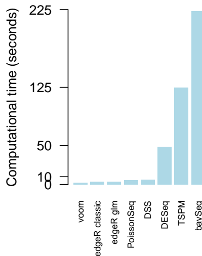
Figure 7: Computing times for RNA-Seq methods. Bars show time in seconds required for the analysis of one simulated dataset on a MacBook laptop. Methods are ordered from quickest to most expensive.
