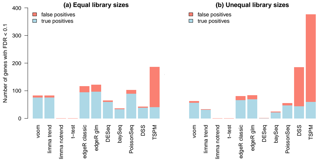
Figure 4: Power to detect true differential expression. Bars show the total number of genes that are detected as statistically significant ( FDR < 0.1 ) (a) with equal library sizes and (b) with unequal library sizes. The blue segments show the number of true positives while the red segments show false positives. The number of genuinely DE genes in this simulation is 200. Results are averaged over 100 simulations. Height of the blue bars shows empirical power. The ratio of the red to blue segments shows empirical FDR.
