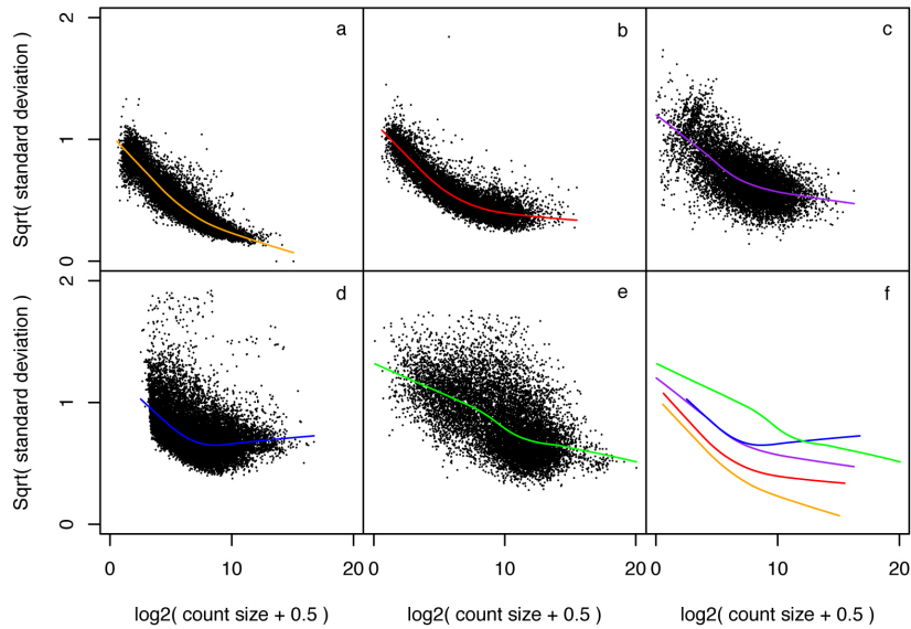
Figure 1: Mean-variance relationships. Gene-wise means and variances of RNA-Seq data represented by black points with a lowess trend. Plots are ordered by increasing levels of biological variation in datasets. Panel (a), voom trend in HBRR and UHRR genes in Sample A, B, C and D of SEQC project; technical variation only. Panel (b), C57BL/6J and DBA mouse experiment; low-level biological variation. Panel (c), simulation study in the presence of 100 up-regulating genes and 100 down-regulating genes; moderate-level biological variation. Panel (d), Nigerian lymphoblastoid cell lines; high-level biological variation. Panel (e), Drosophila melanogaster embryonic developmental stages; very high biological variation due to systematic differences between samples. Panel (f), lowess voom trends for datasets a–e.
